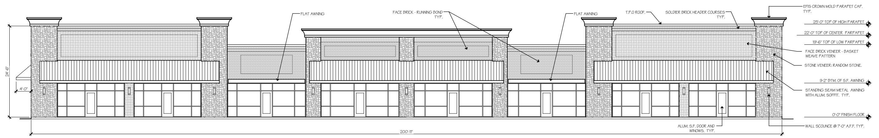
FRONT ELEVATION
