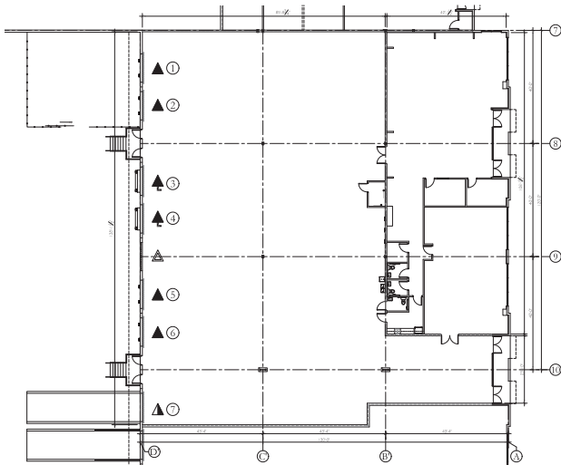
Overall Floorplan - 17,938 SF
