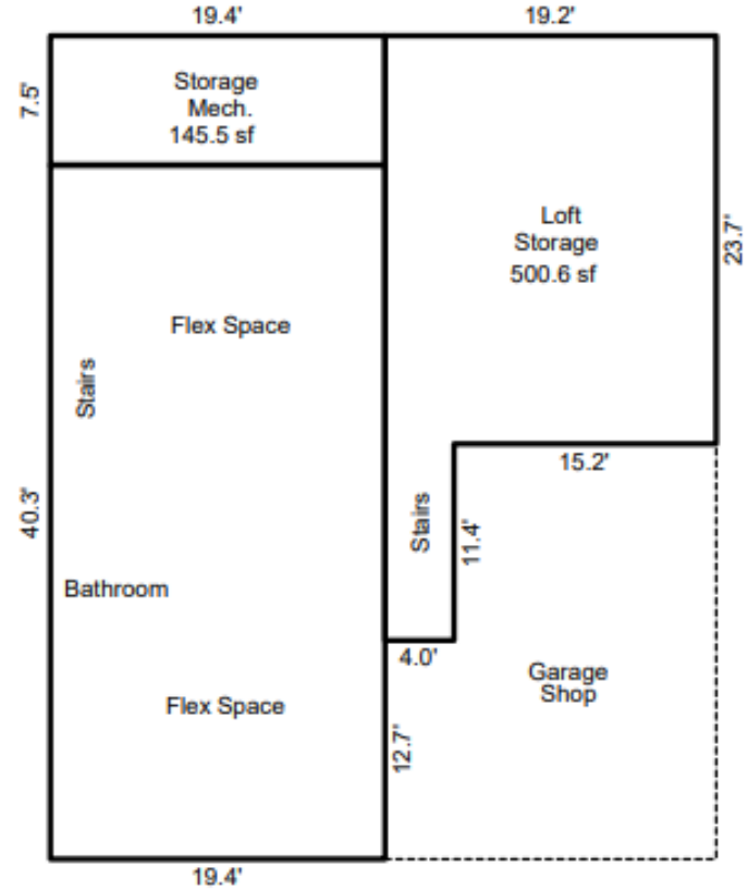
Second Floor 781.8 sf
