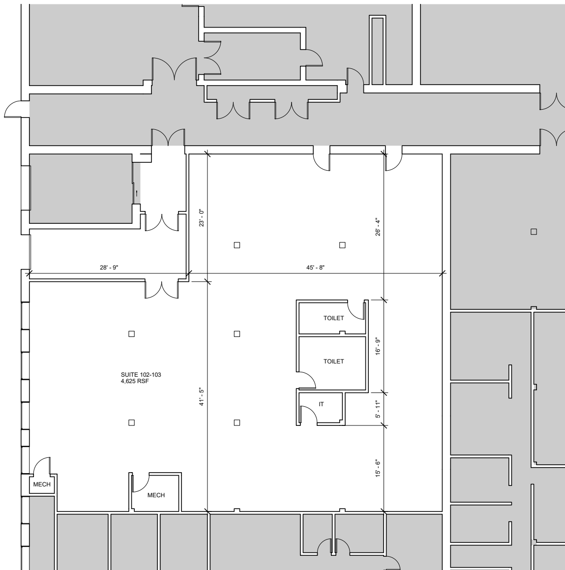
① SUITE 102-103 1/8" = 1'-0"
