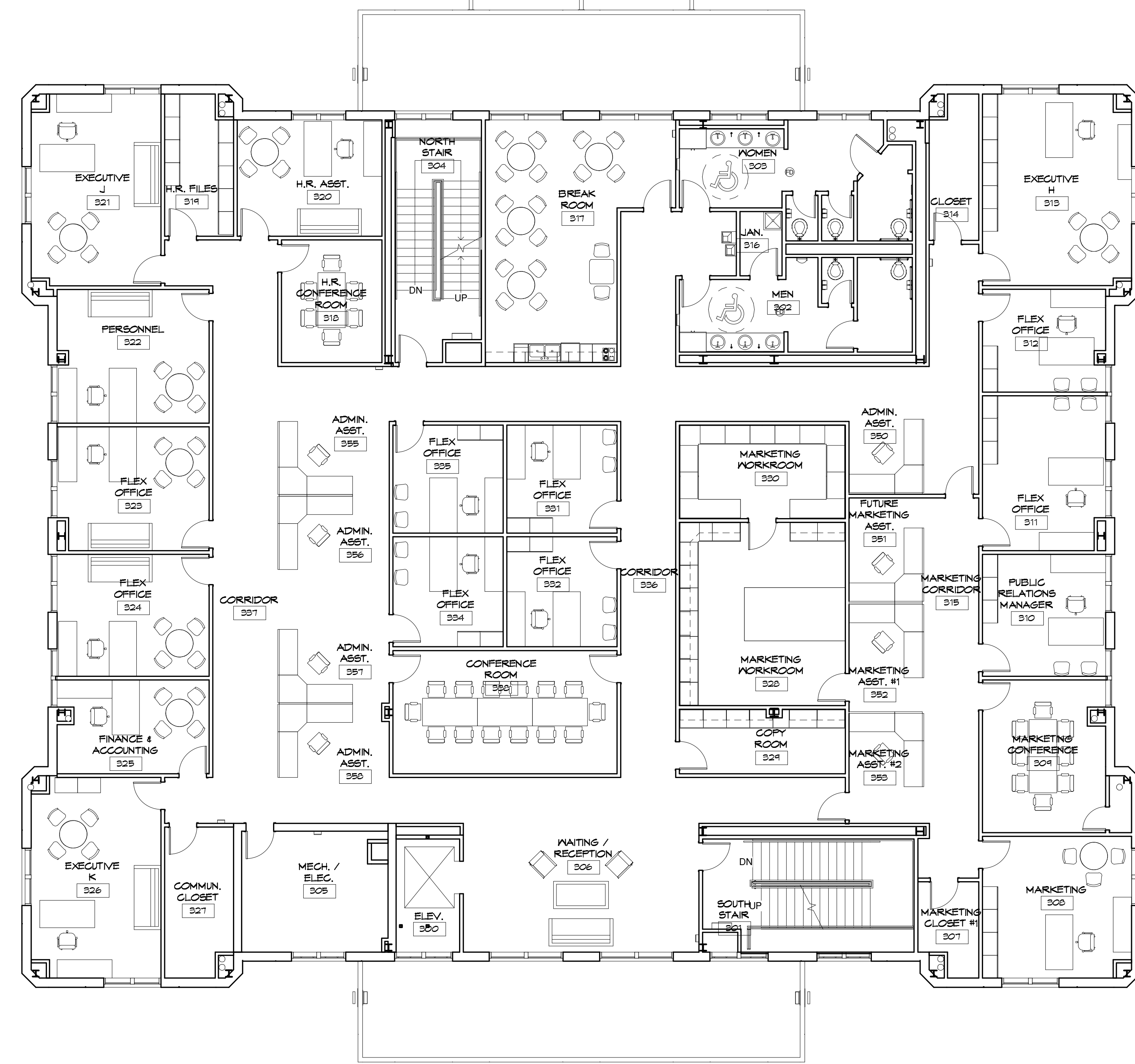
A3 A1 | A5.11 1/8" = 1'-0" THIRD FLOOR FURNITURE PLAN 11,271 GROSS SQUARE FOOTAGE
