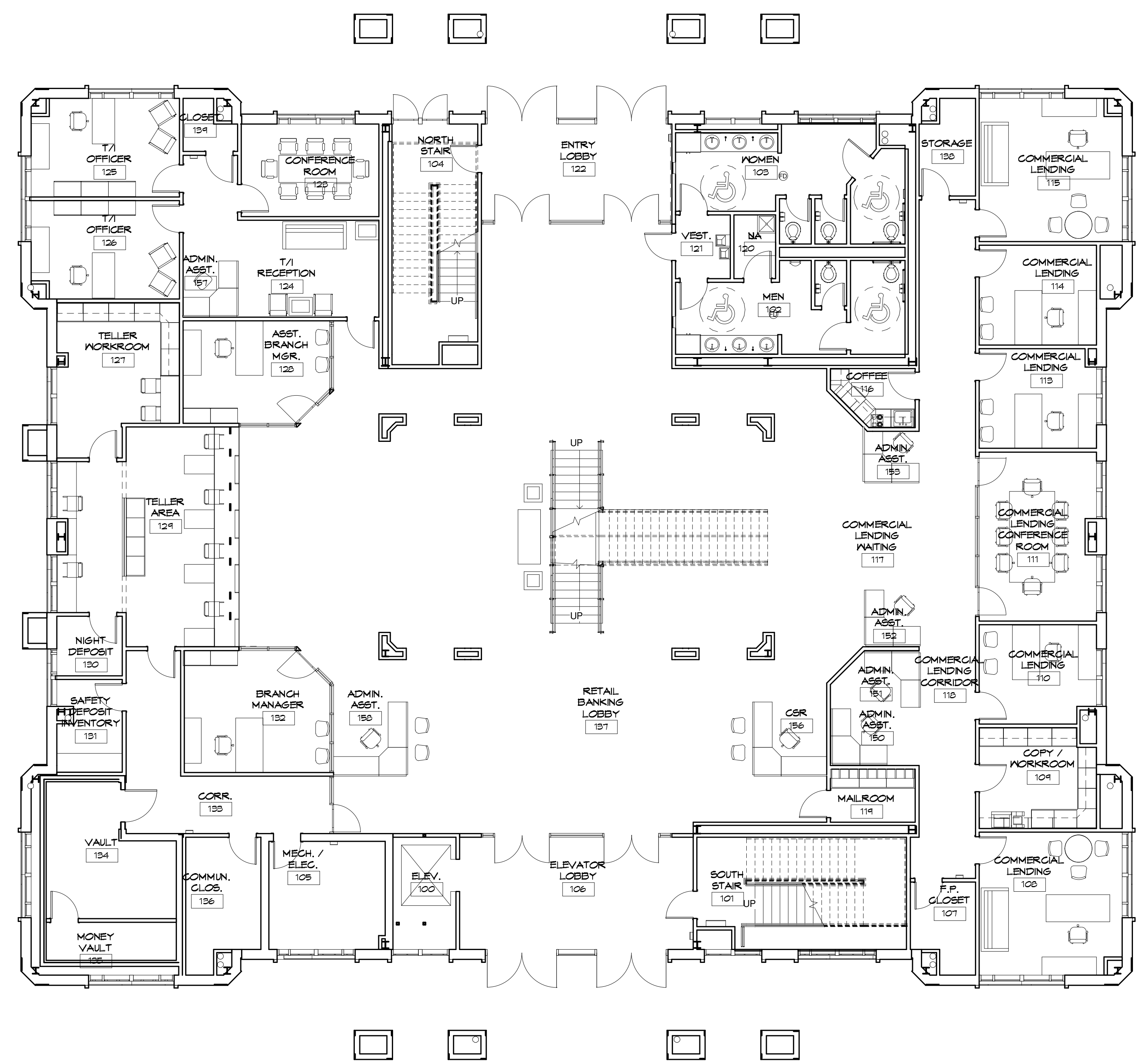
A3 A1 | A5.11 | FIRST FLOOR FURNITURE PLAN 11,271 GROSS SQUARE FOOTAGE 1/8" = 1'-0"
