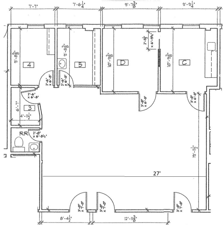
Second Floor Plan - 1,087 SF (Unit 210)
