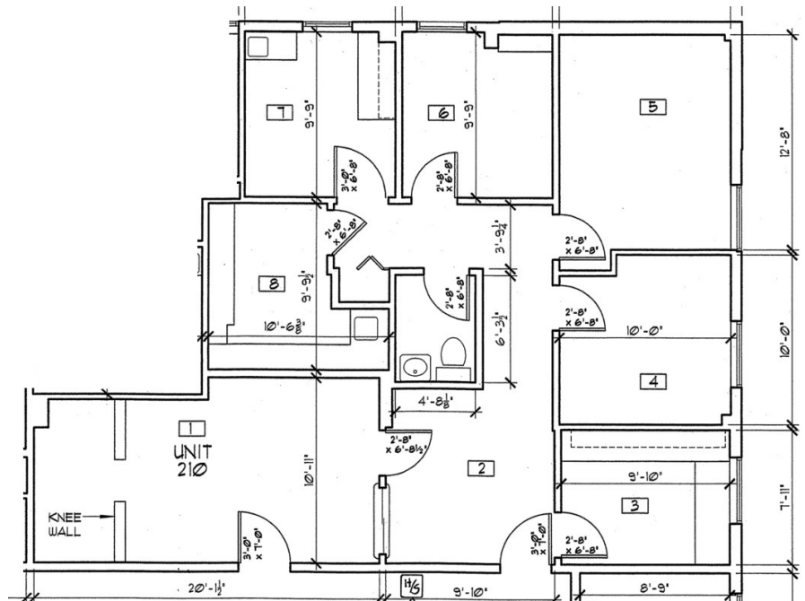
Second Floor Plan - 1,087 SF (Unit 210)
