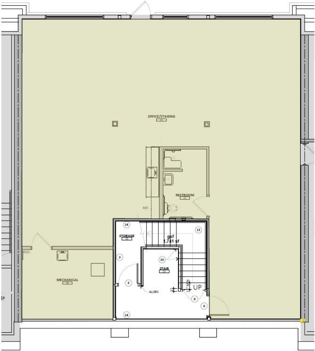
2 LOWER LEVEL FLOOR PLAN A100 1/4" = 1'-0"
