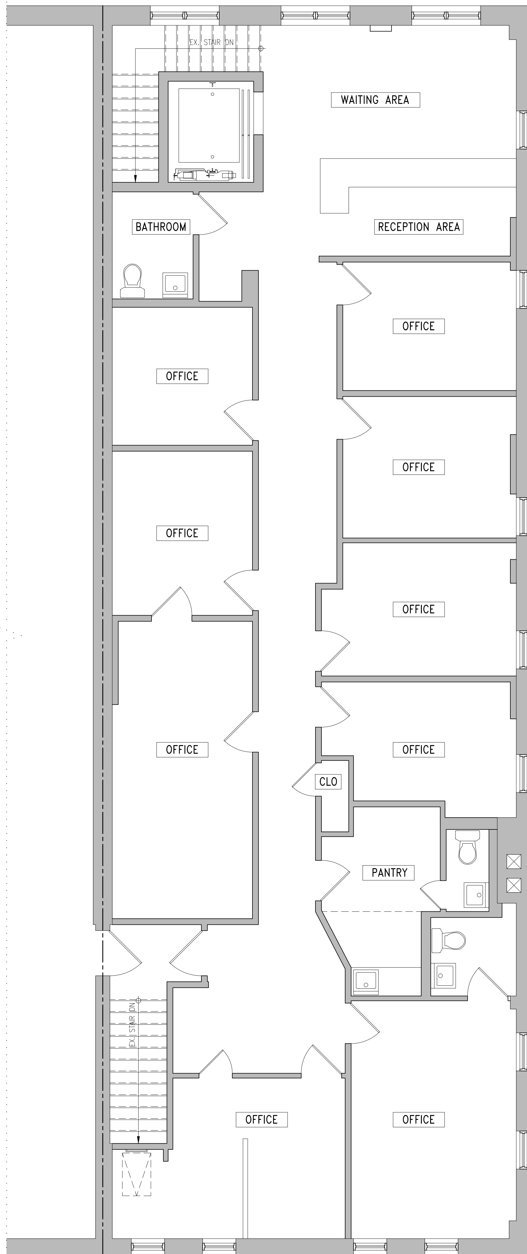
EXISTING SECOND FLOOR PLAN
