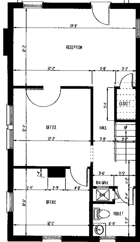
446 FIRST FLOOR PLAN
