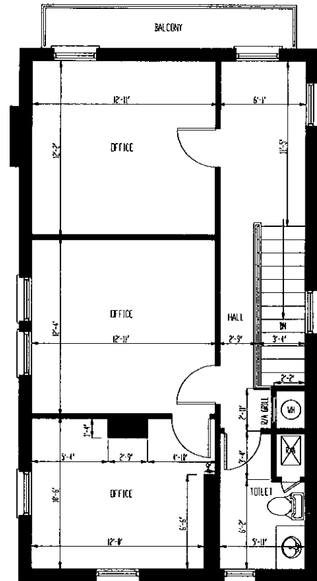
446 SECOND FLOOR PLAN
