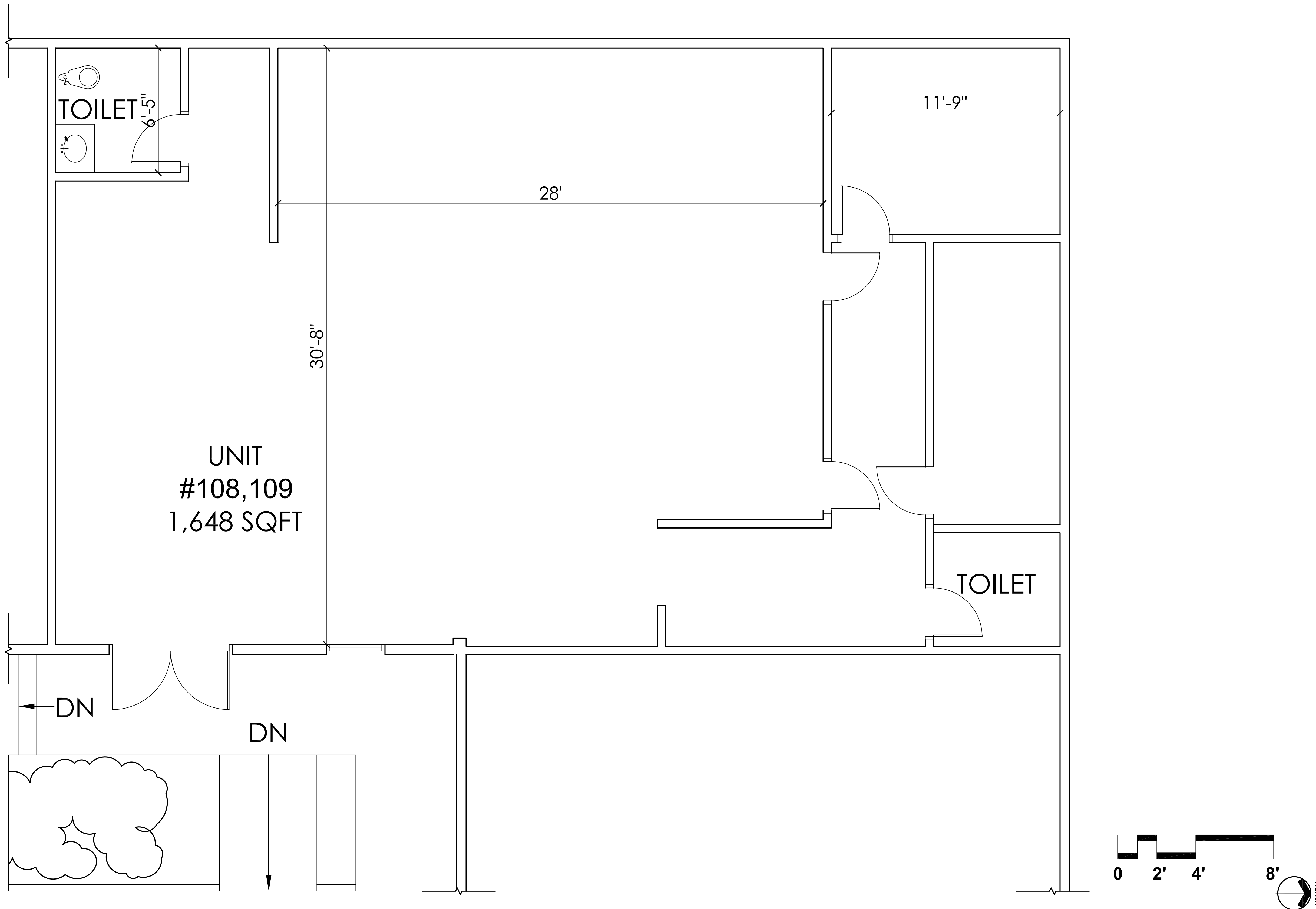
1 FLOOR PLAN Scale: 3/8"=1'-0"
