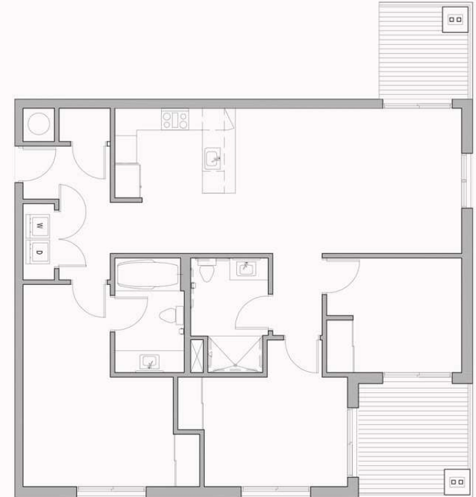
Type C floor plan 3 bedrooms 2 baths 1,580 SF 100 SF private balconies
