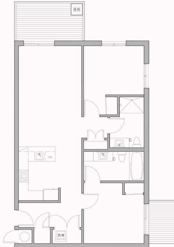
Type B floor plan 2 bedrooms 2 baths 1,150 SF 100 SF private balconies
