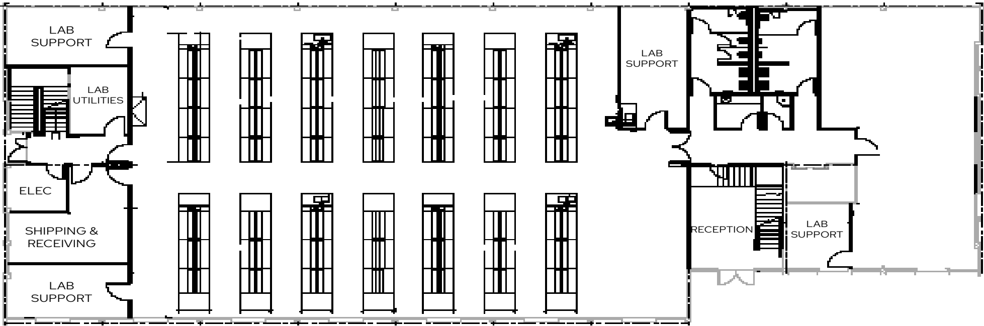
First Floor
