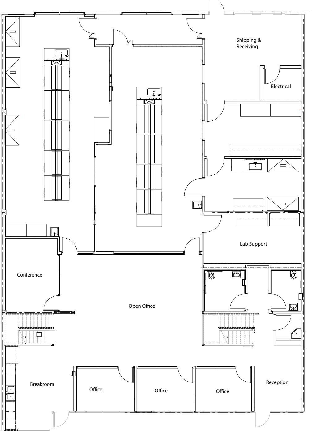
First Floor
