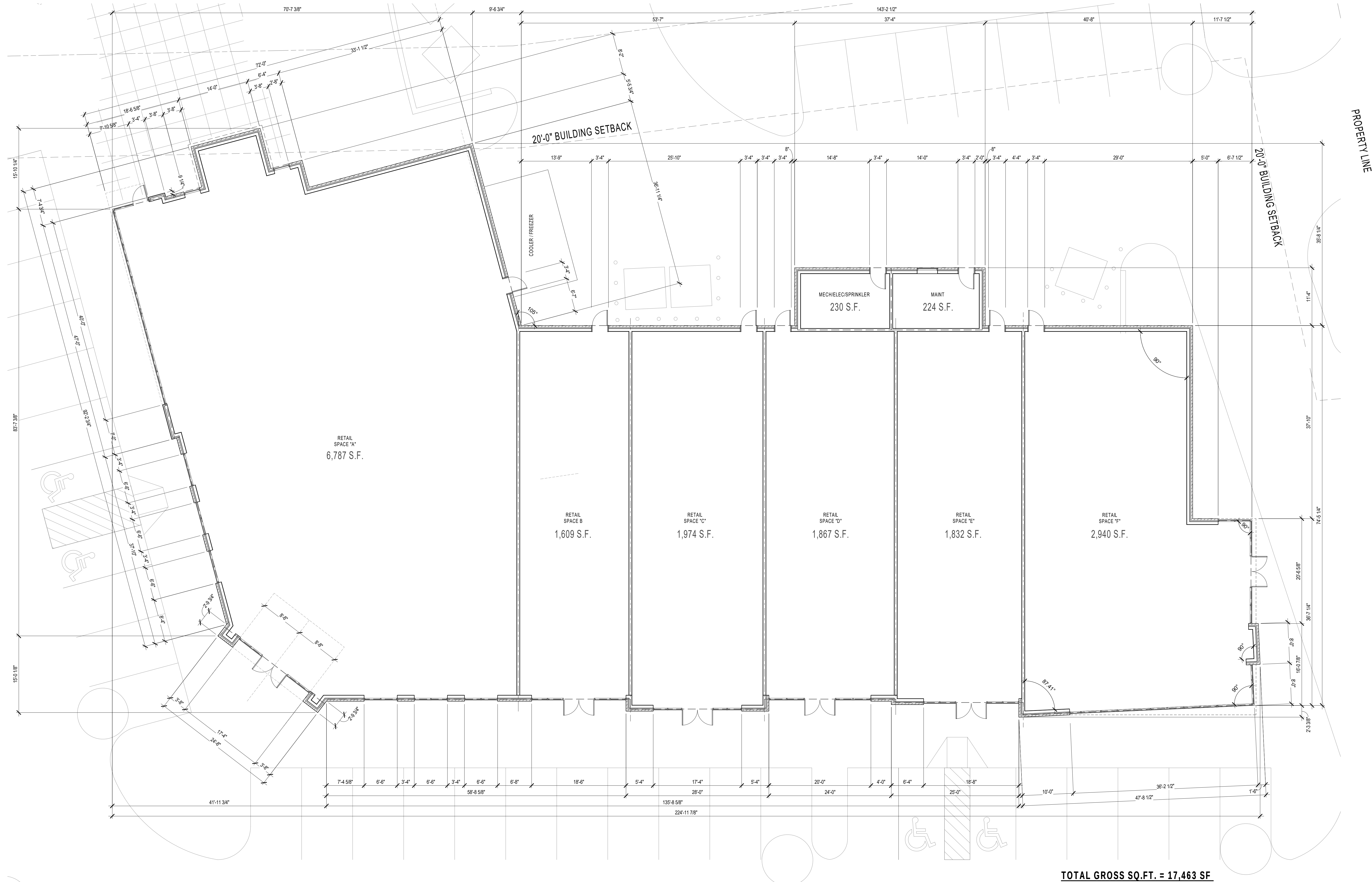
1 FIRST FLOOR 1/8" = 1'-0"
