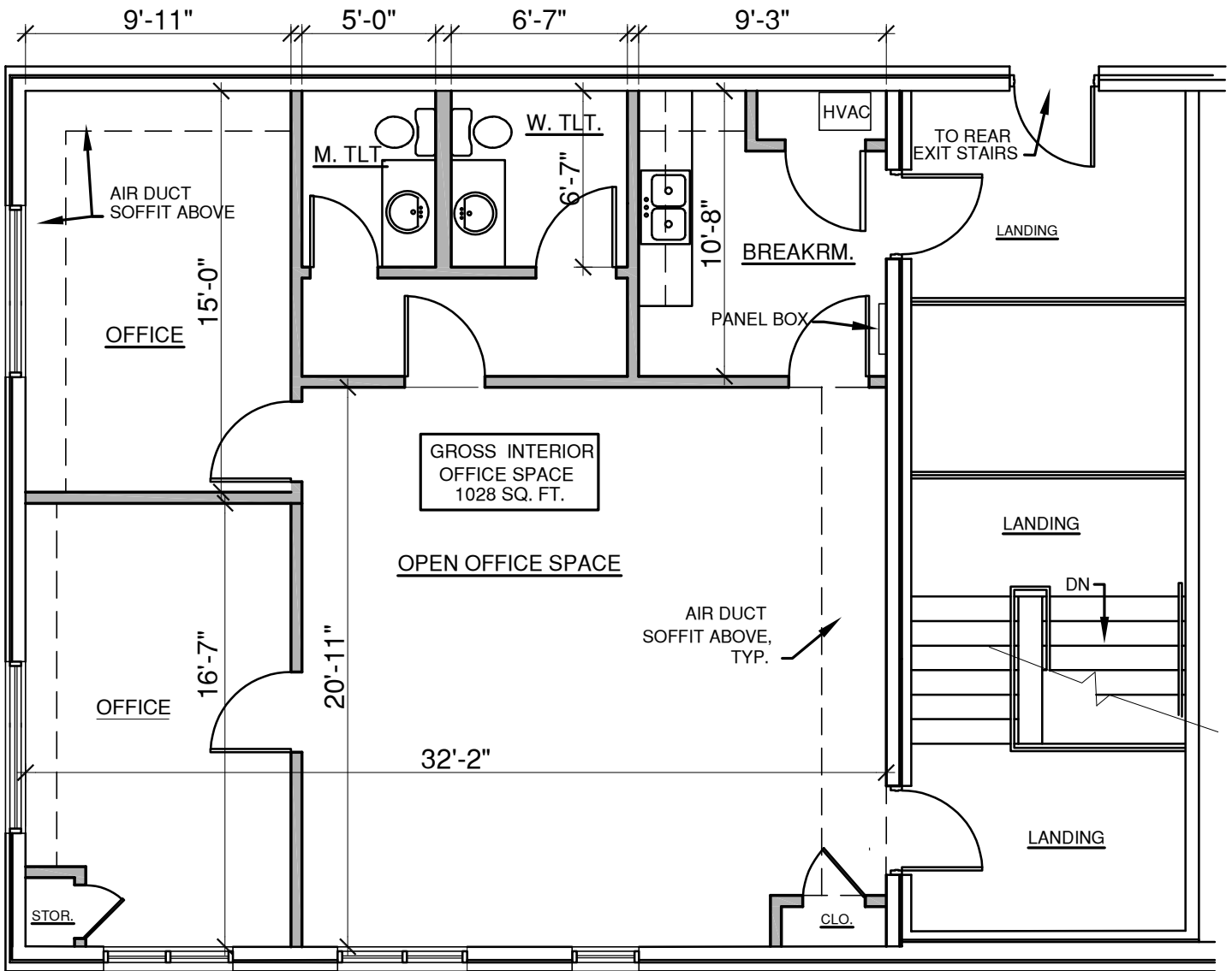
SUITE 209 FLOOR PLAN - EXISTING CONDITIONS 2701 GREYSTONE ROAD, SUITE C NASHVILLE, TN 37204
