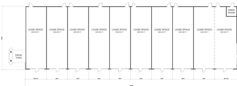
PROPOSED FLOOR PLAN SCALE: 1/8"=1'-0"
