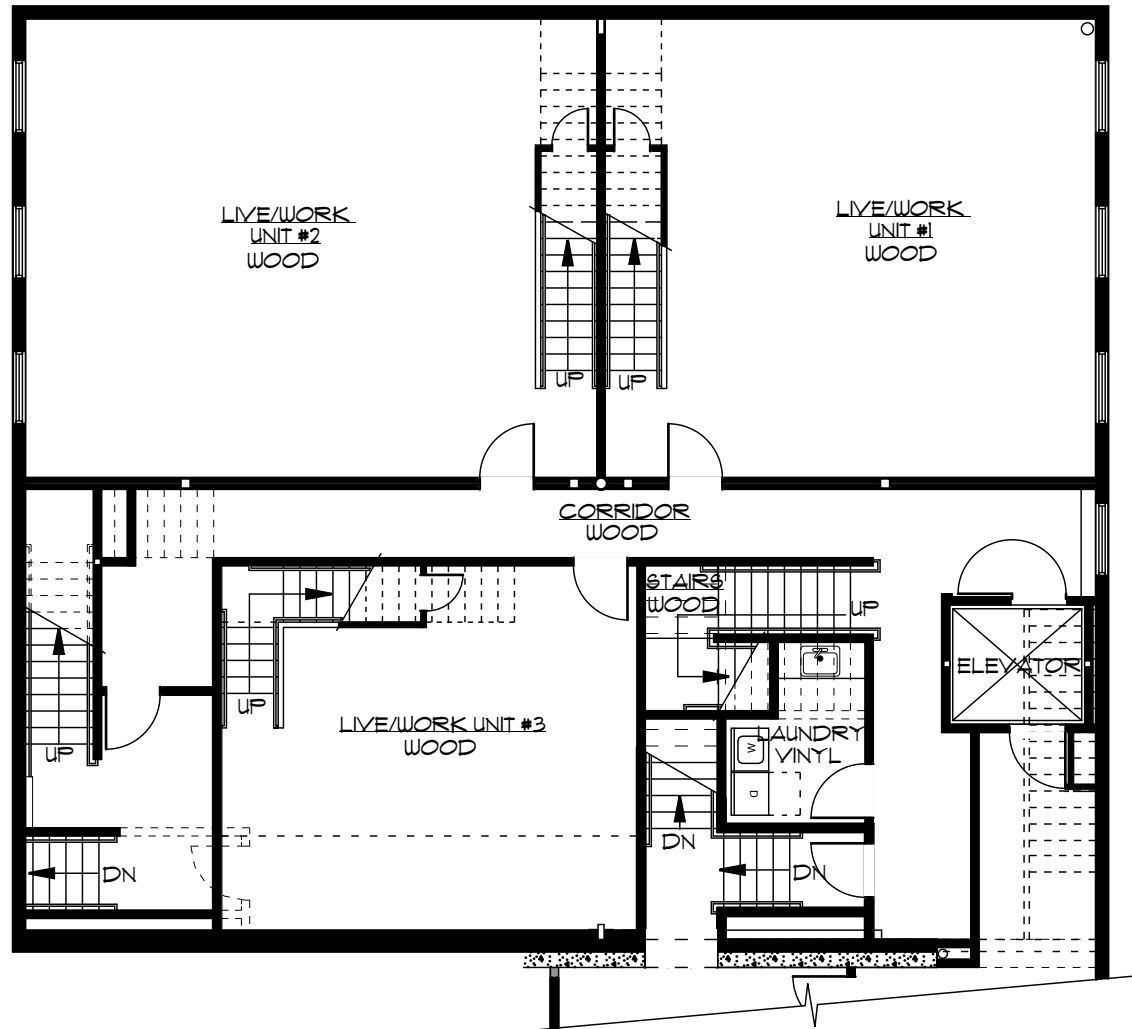
A 2ND FLOOR PLAN - LEVEL 'B' A8 NTS
