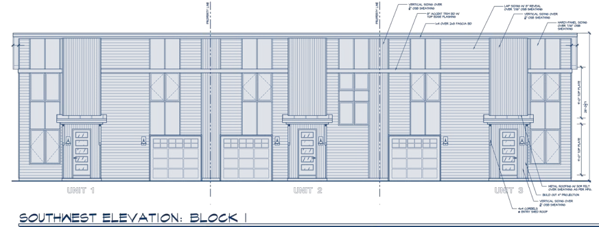
SOUTHWEST ELEVATION: BLOCK 1
