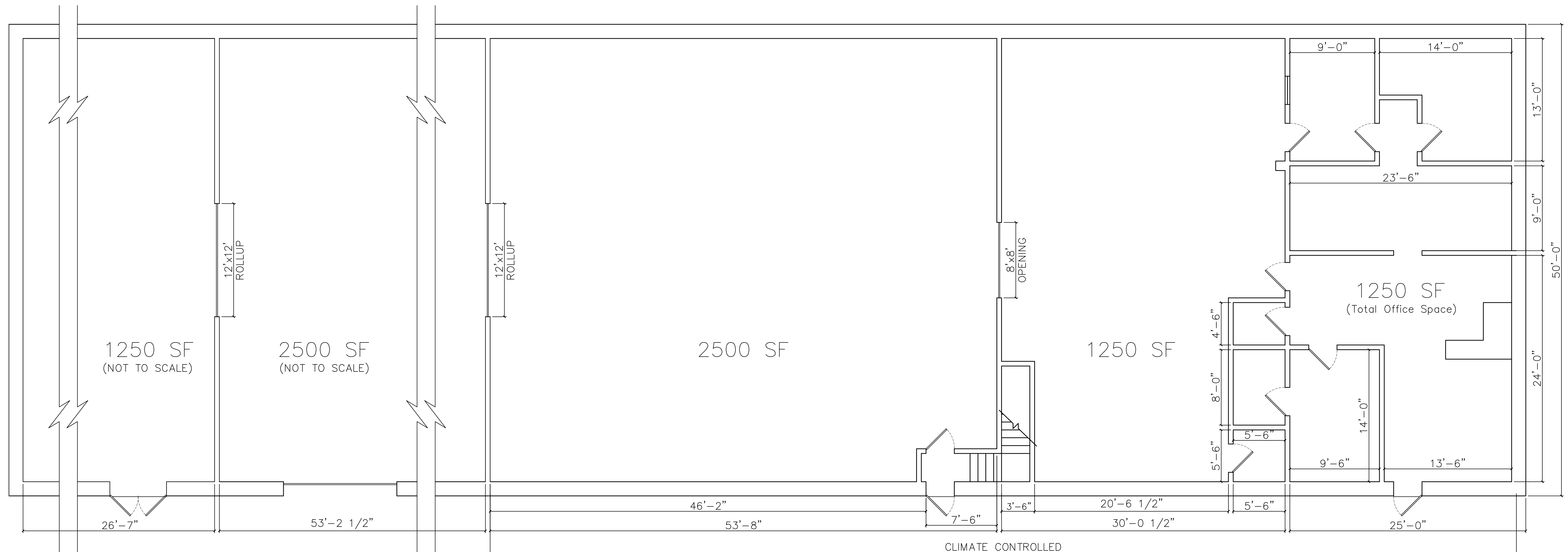
First Floor SCALE: 3/16" = 1'-0"
