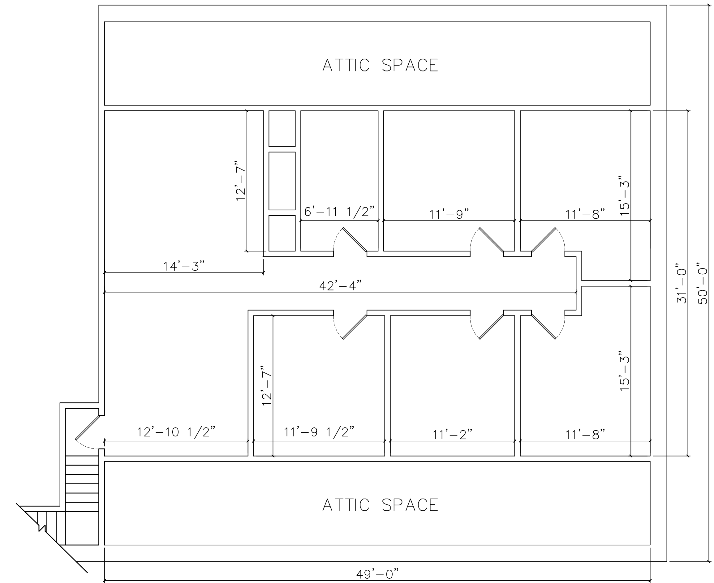
Second Floor SCALE: 3/16" = 1'-0"
