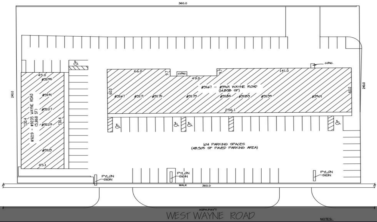
Site Plan
