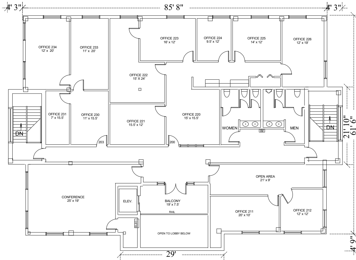
2060 FT. HENRY DR., KINGSFORT, TN UPPER LEVEL - 5,566 SQUARE FEET
