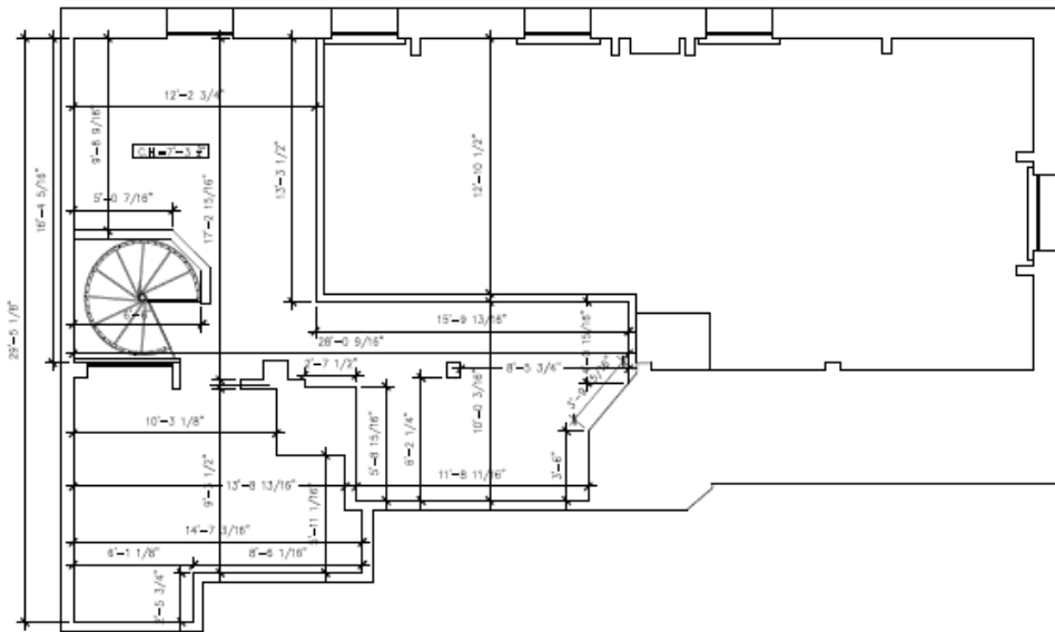
MEZZANINE
