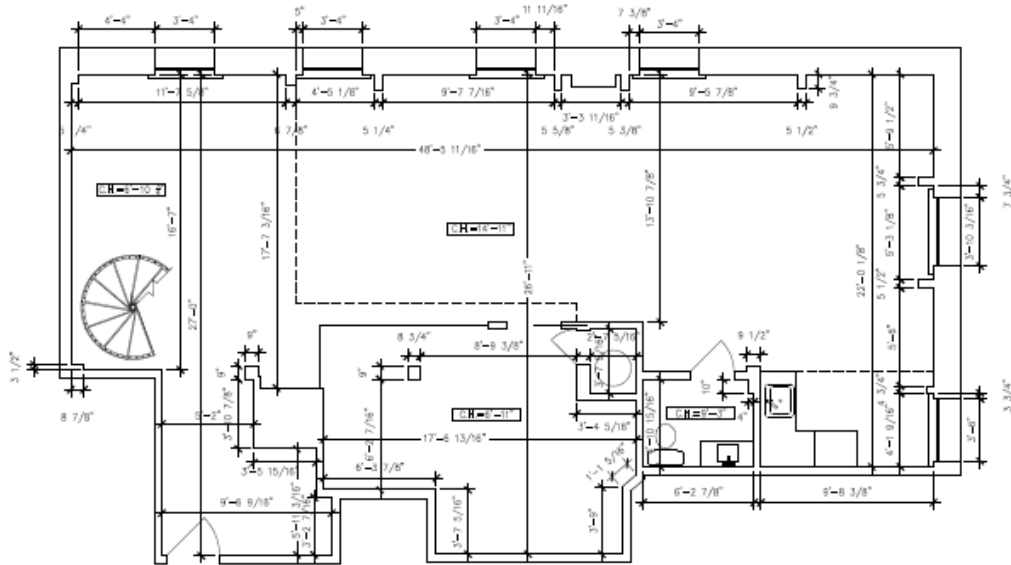
GROUND FLOOR
