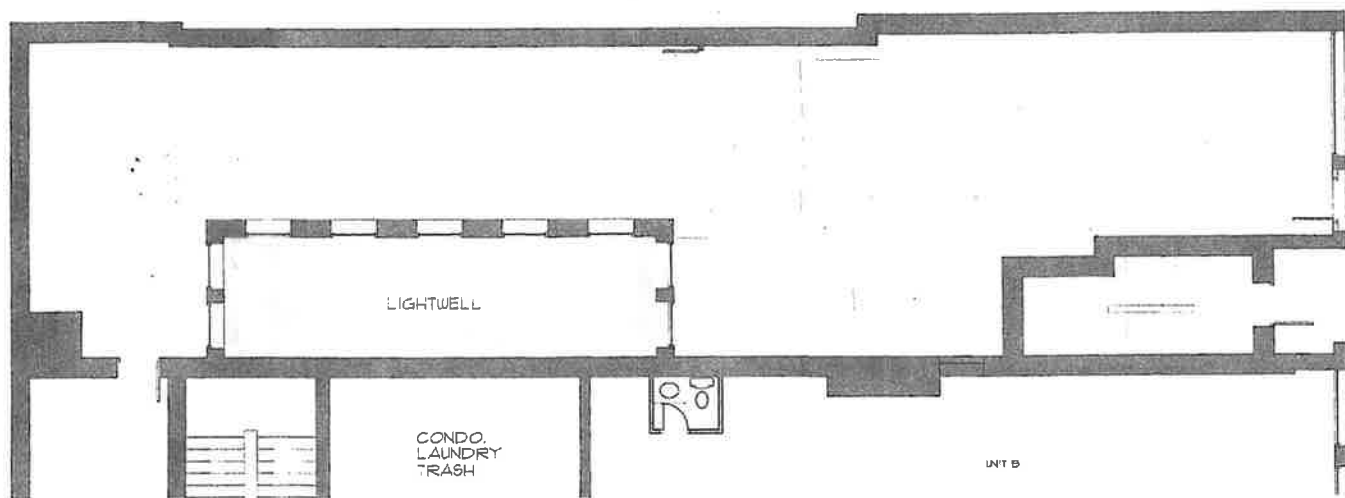
1 SCHEMATIC FLOOR PLAN - UNIT C SCALE: 1/4" = 1'-0"
