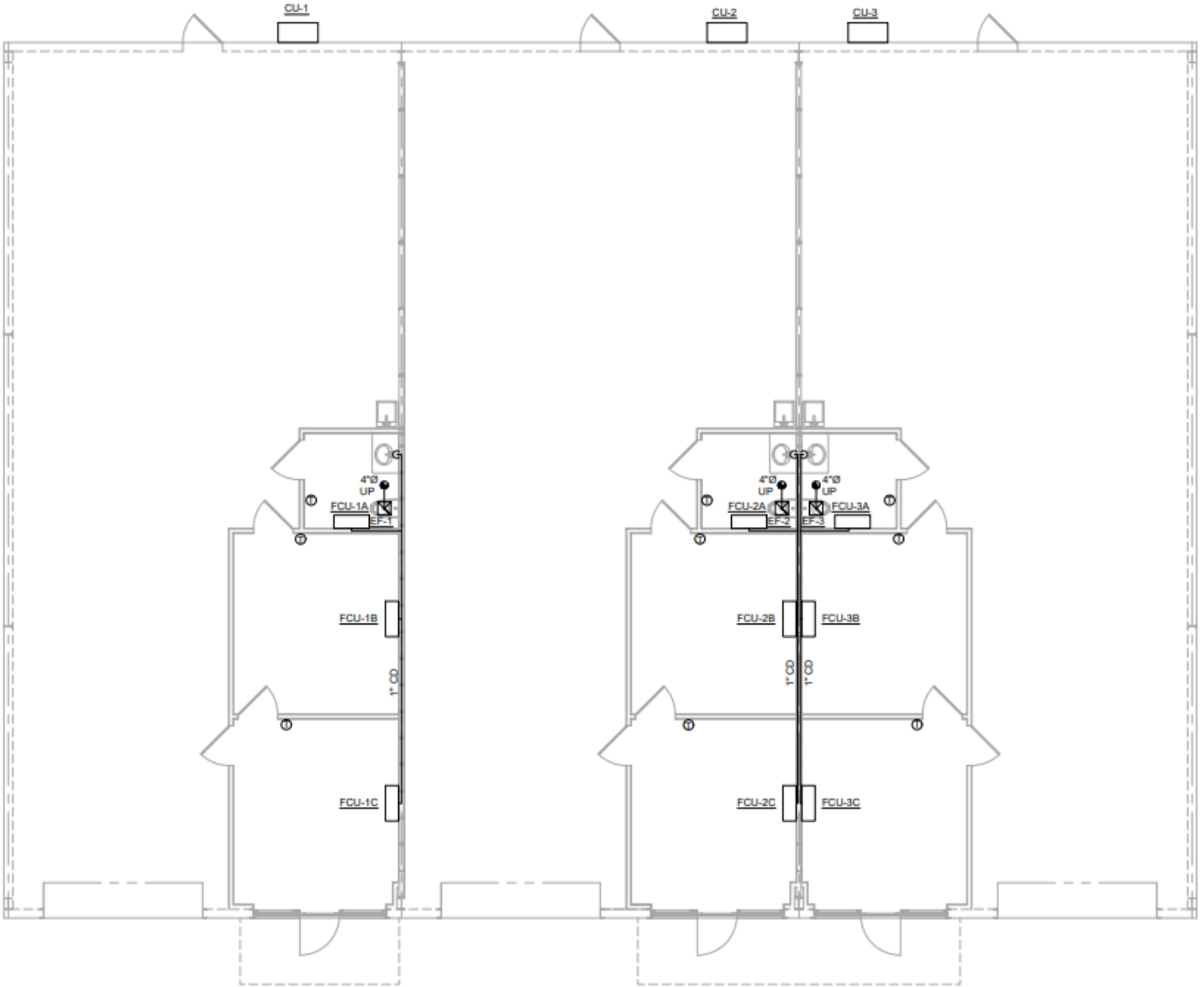
1 MECHANICAL FLOOR PLAN 3/16" = 1'-0"
