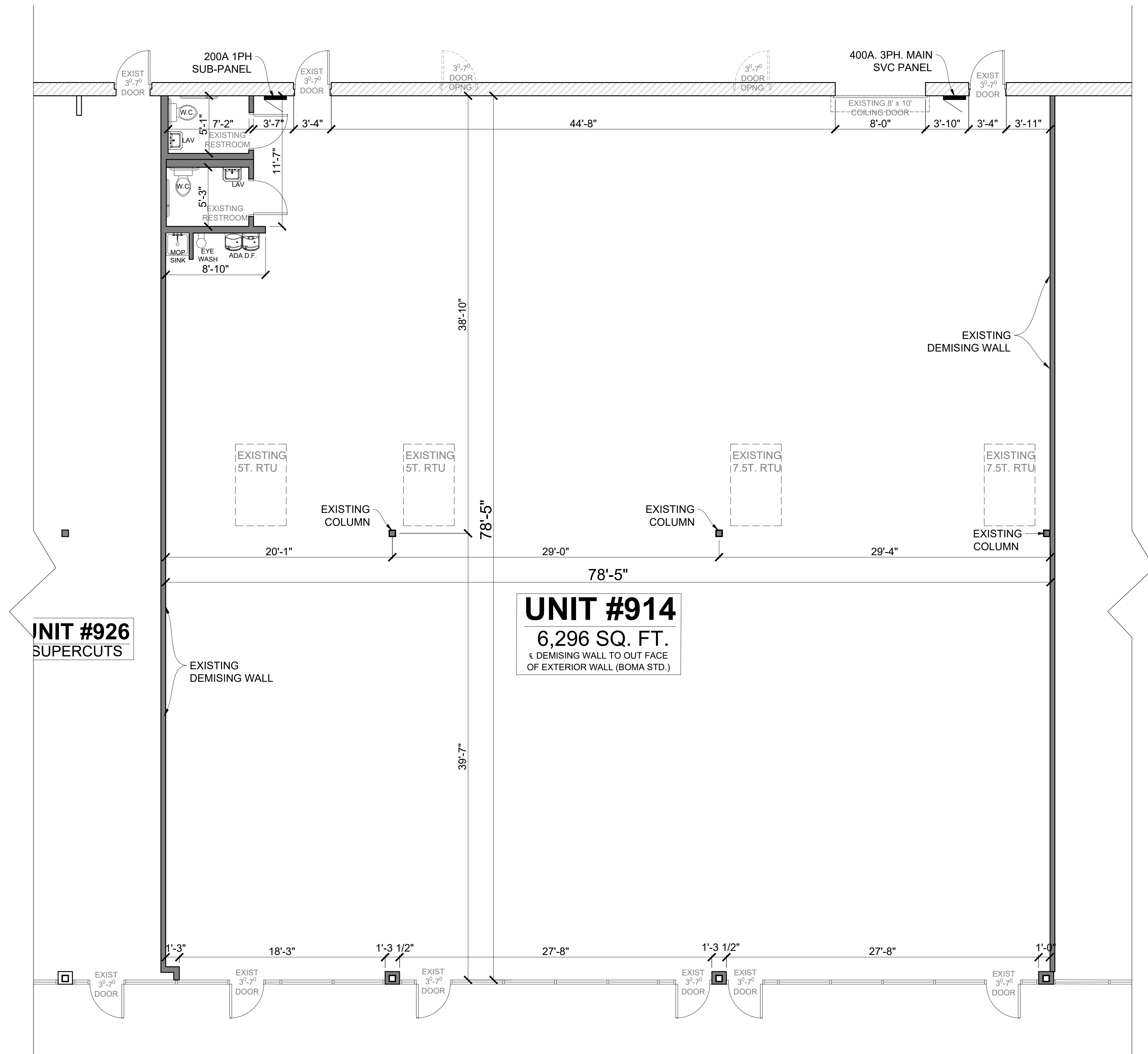
1 UNIT #914 - LEASE AREA PLAN SCALE: 3/16" = 1'-0"
