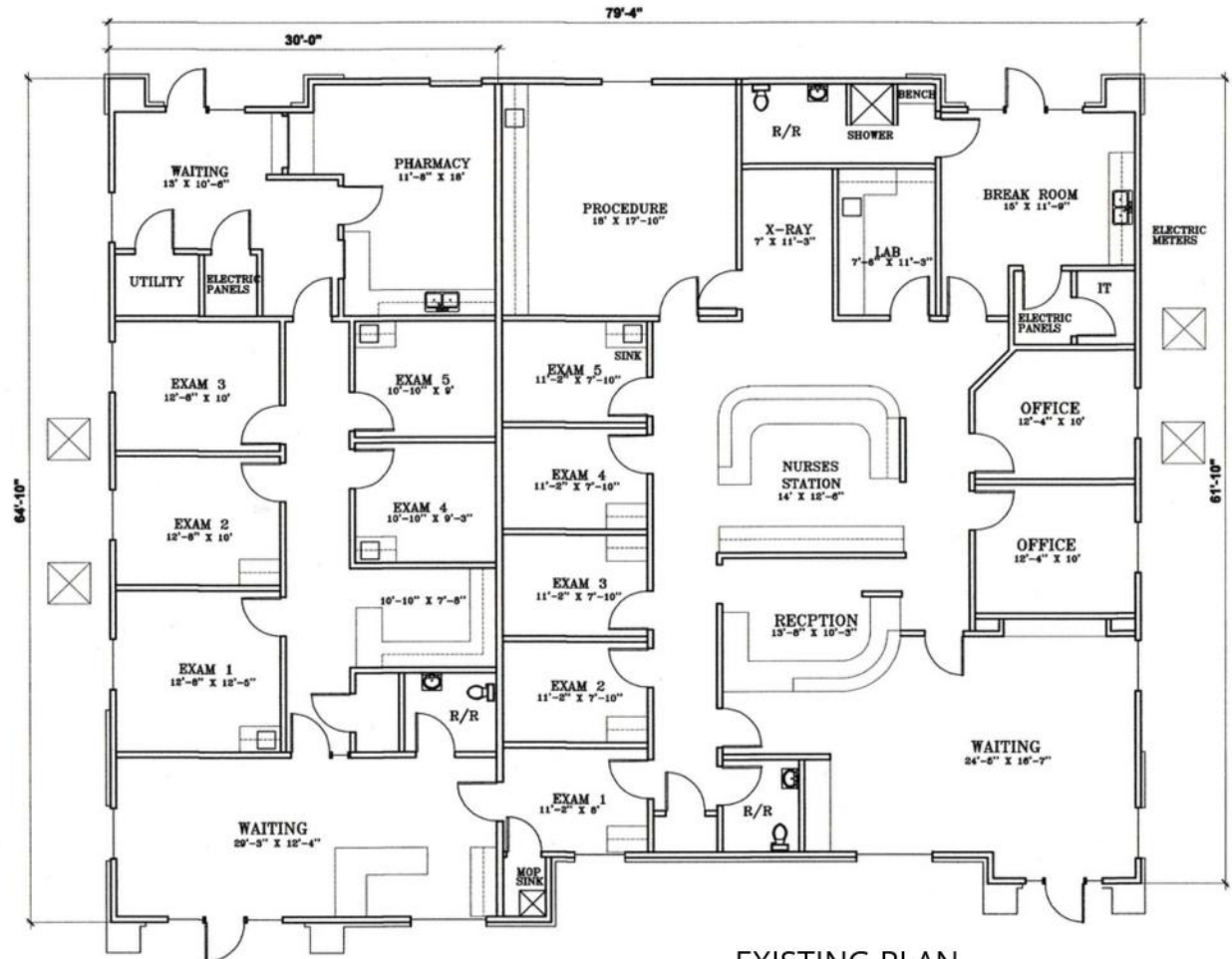
EXISTING PLAN SUITE 400 2,994 SF
