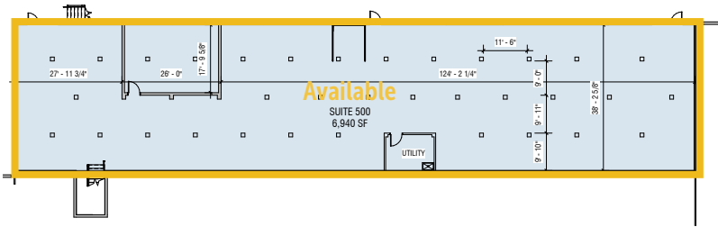
2 A000 BASEMENT LEASING SCALE: 1/16" = 1'-0"
