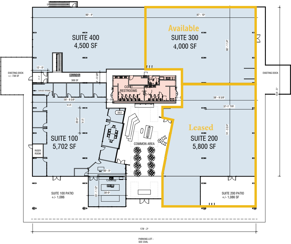
1 A000 FIRST FLOOR - LEASING SCALE: 1/16" = 1'-0"
