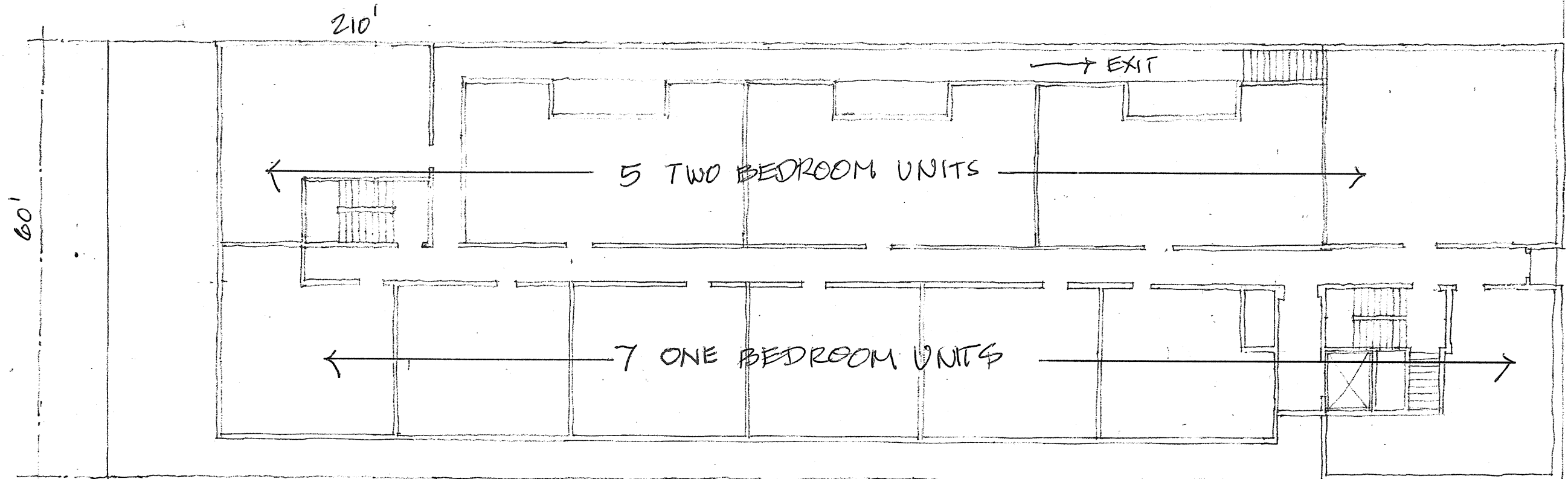
SECOND FLOOR PLAN 1"=16'
