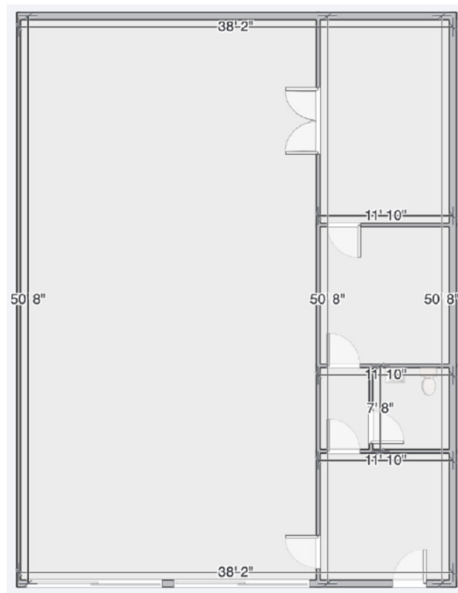
Office with 2 Bays
