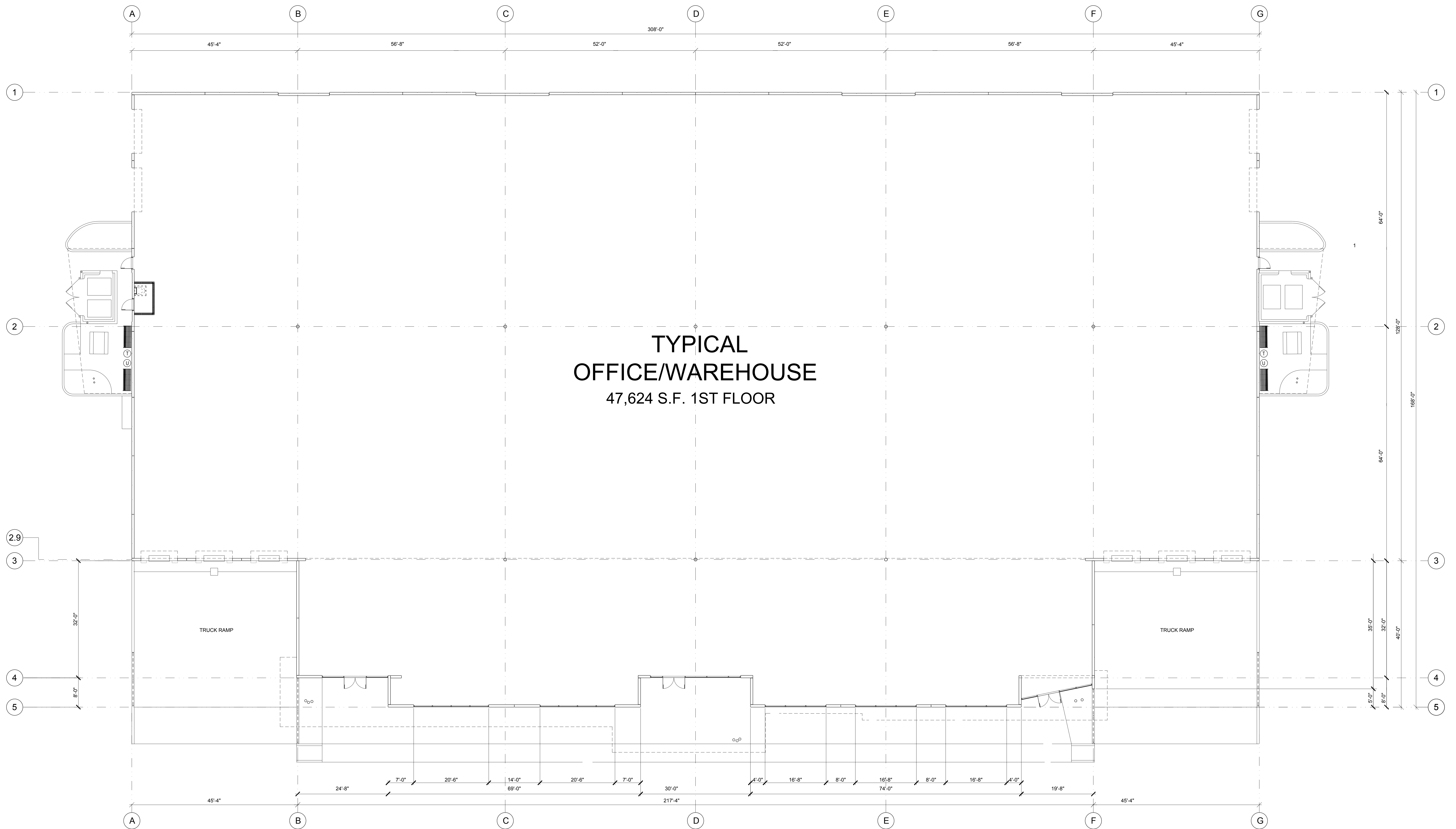
1 Floor Plan - Buildings 'A' & 'C'
