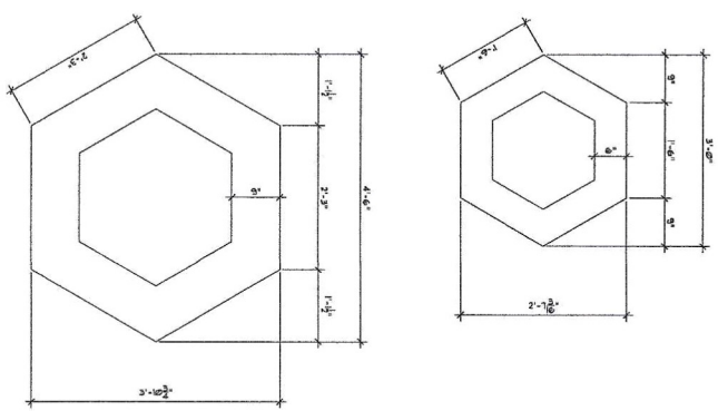
2 ENLARGED HEXAGON PLAN A2.1 1" = 1'-0"
