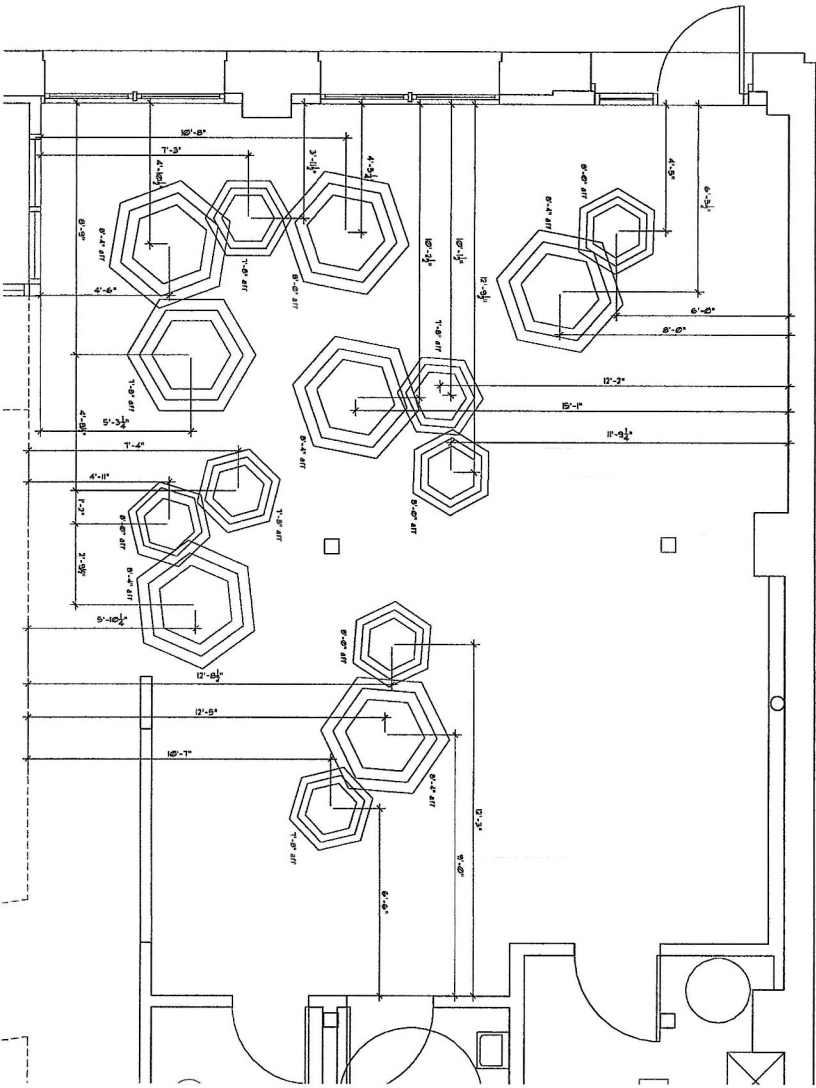
1 CAFE DETAILED REFLECTED CEILING PLAN A2.1 1/2" = 1'-0"
