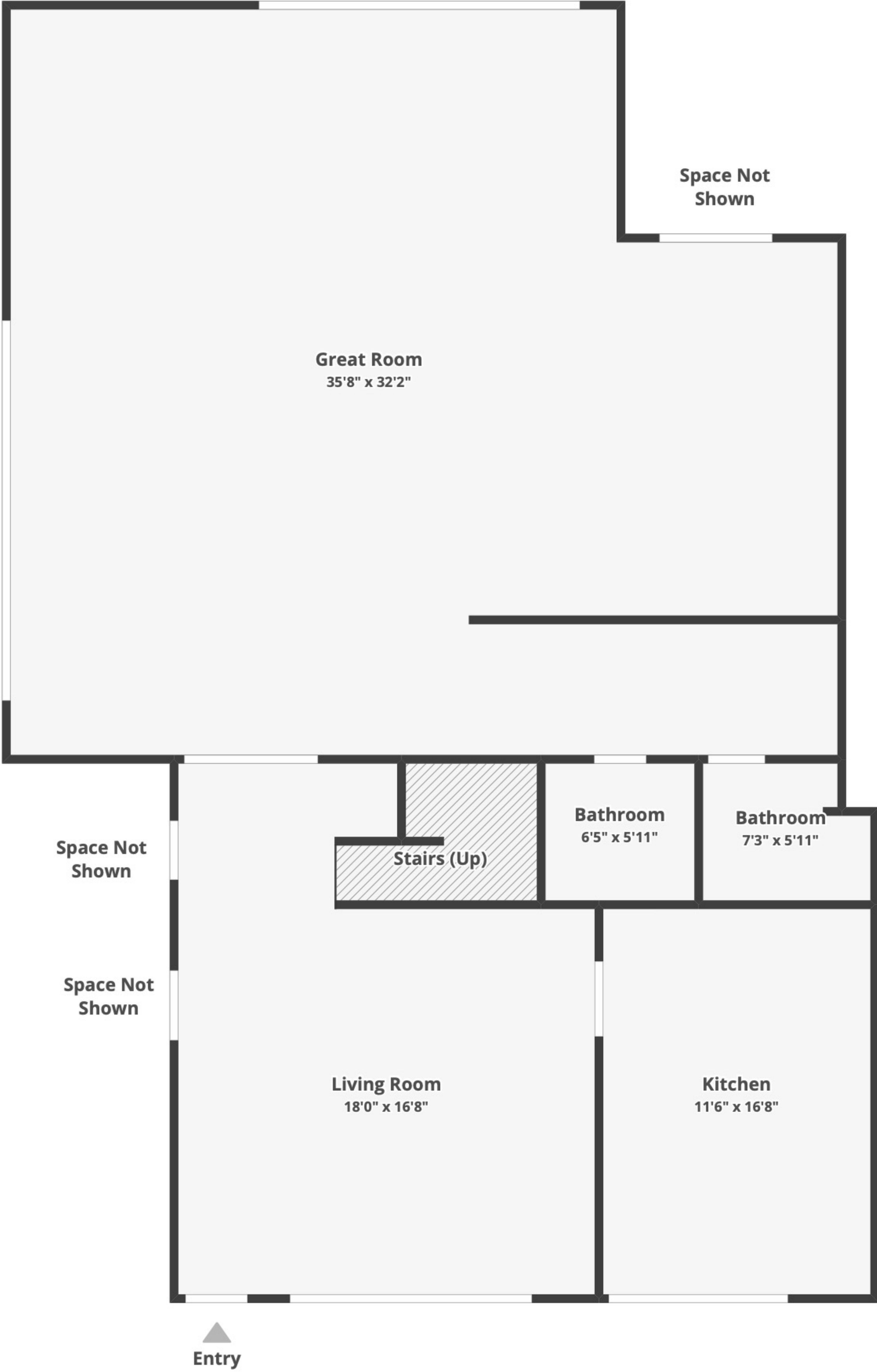
FLOOR 1
