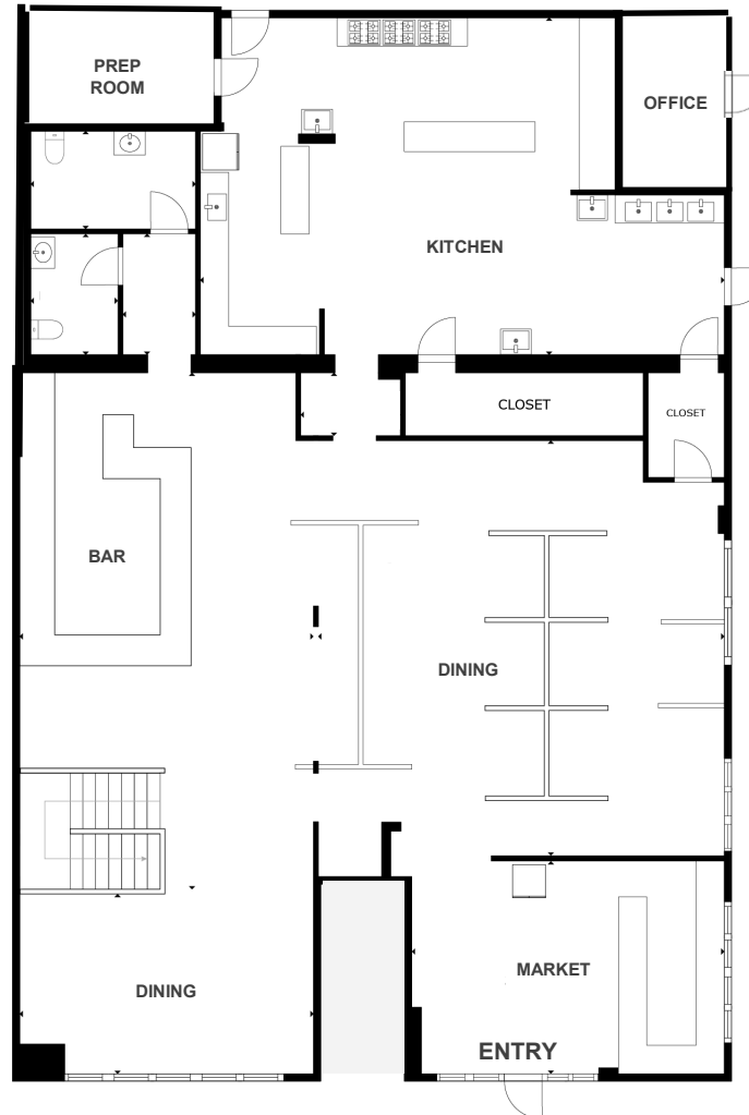
MAIN FLOOR
