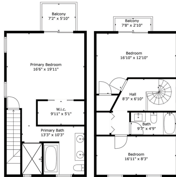
Second Level
