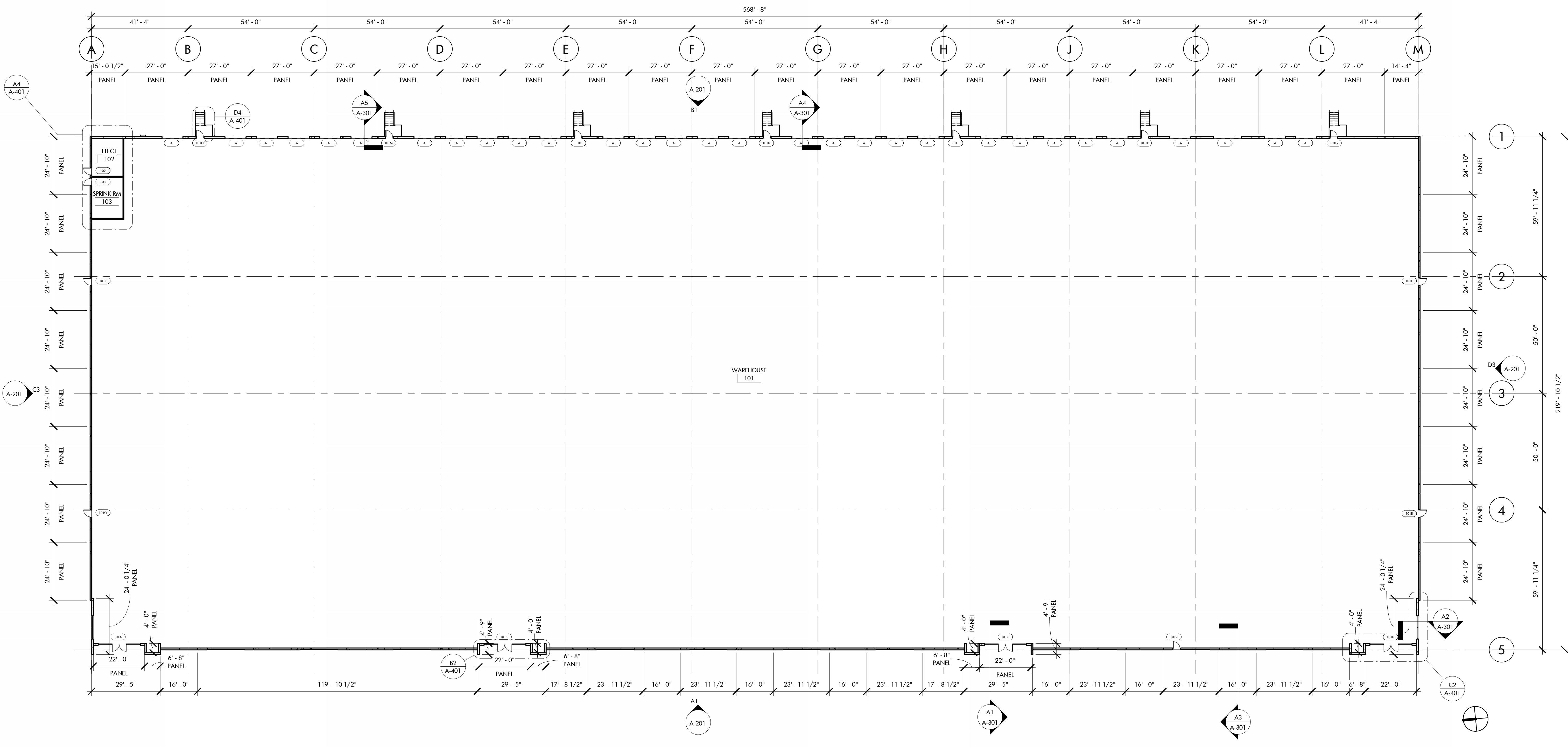
A1 LEVEL 1 PLAN A-101 3/64" = 1'-0"
