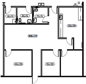
OFFICE PLAN
