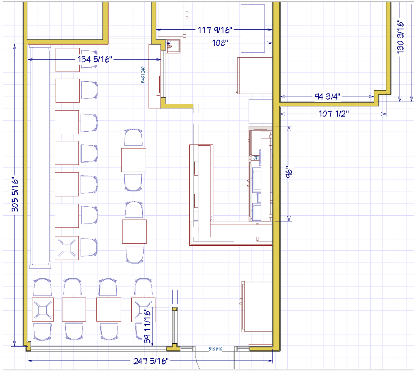
General Floorplan (1 of 2)
