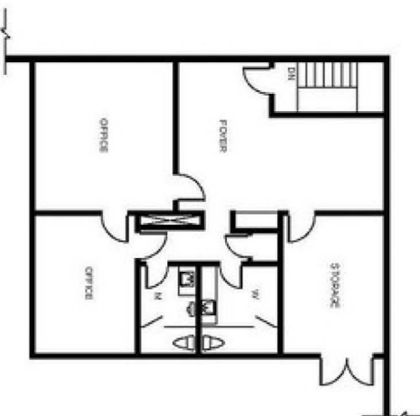
MEZZANINE PLAN
