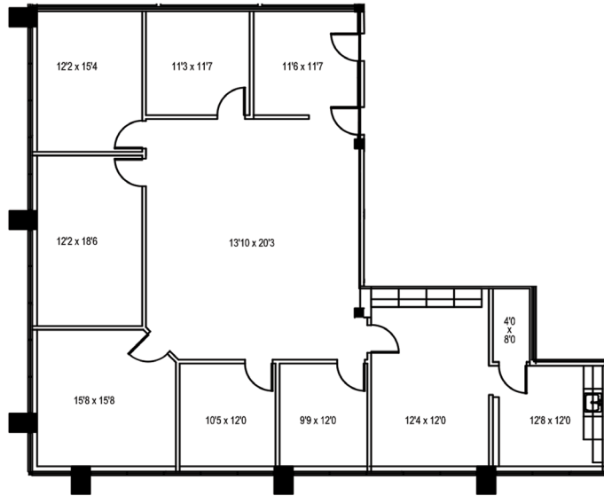
Suite 300: 2,589 SF
