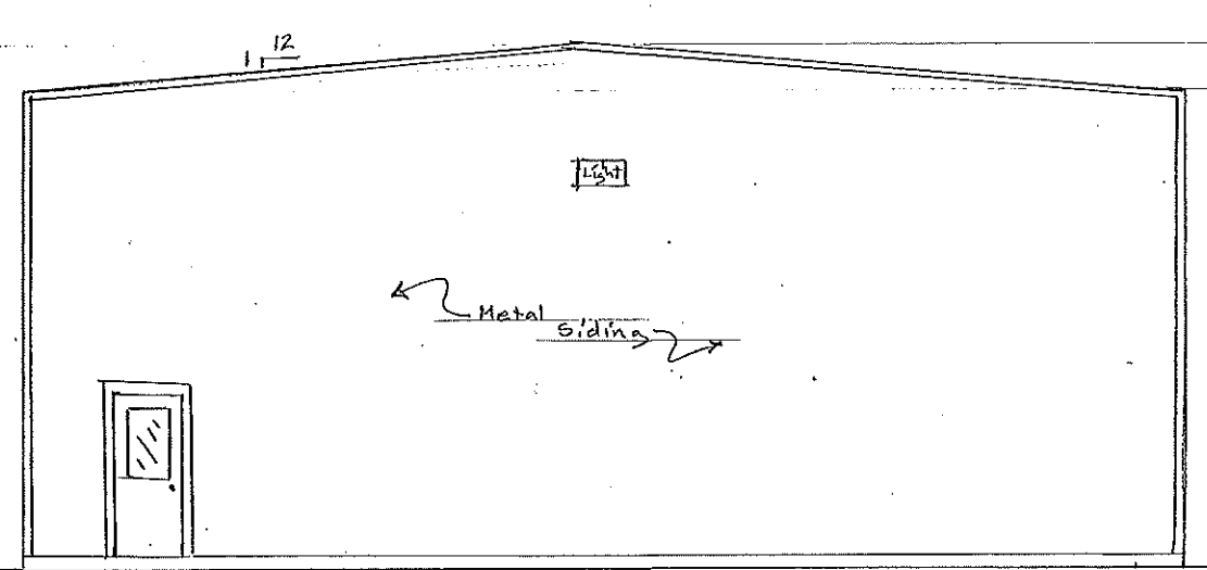
Rear View Scale: 1/4"=1'-0"
