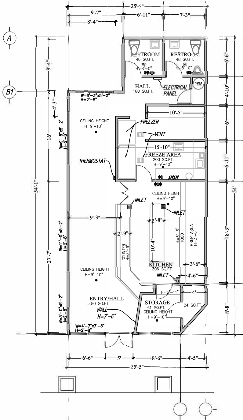
FLOOR PLAN SCALE: 3/32" = 1'- 0"
