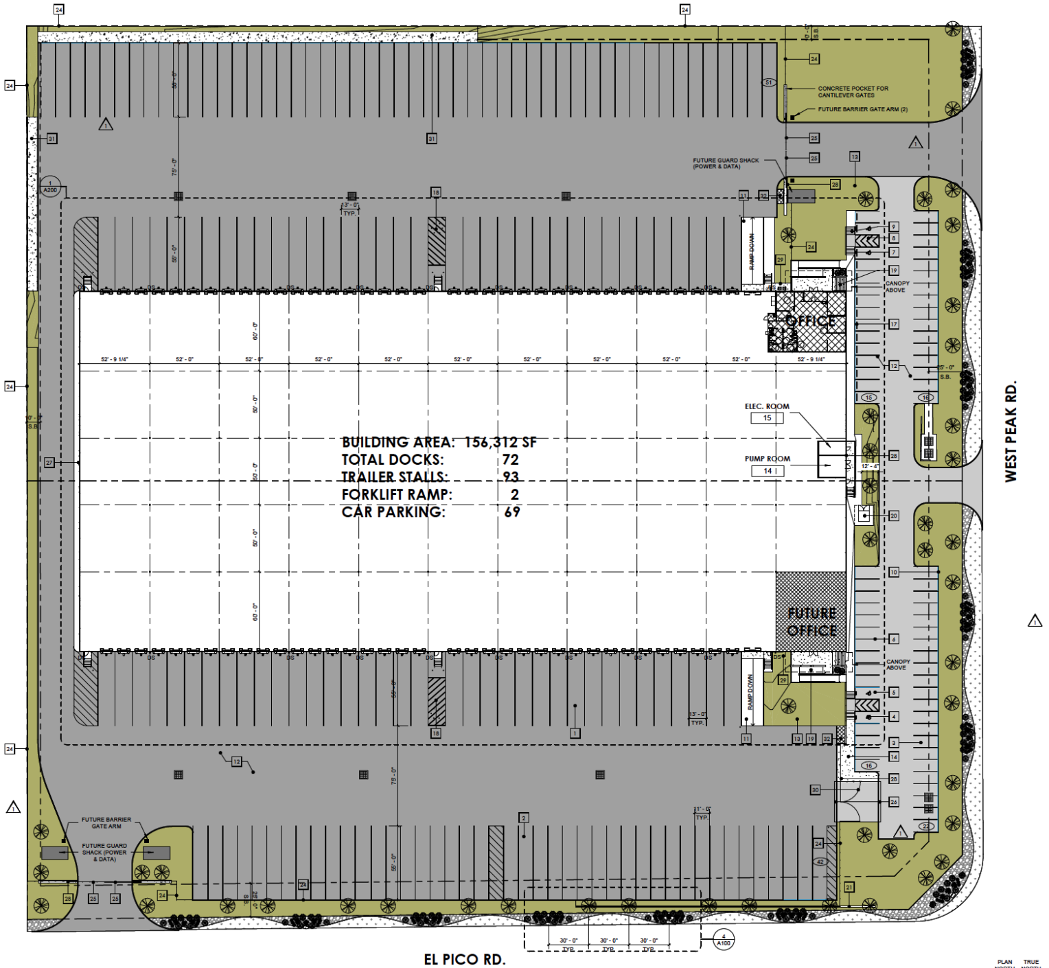
1 SITE PLAN - PLAN NORTH 1/32" = 1'-0"
