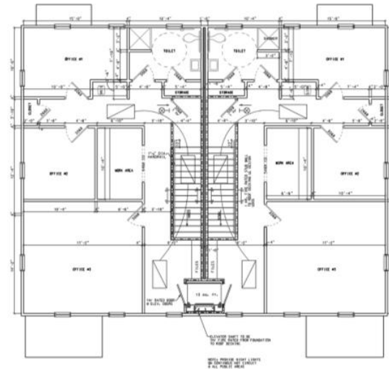
second level floor plan
