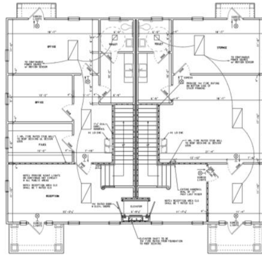
first level floor plan
