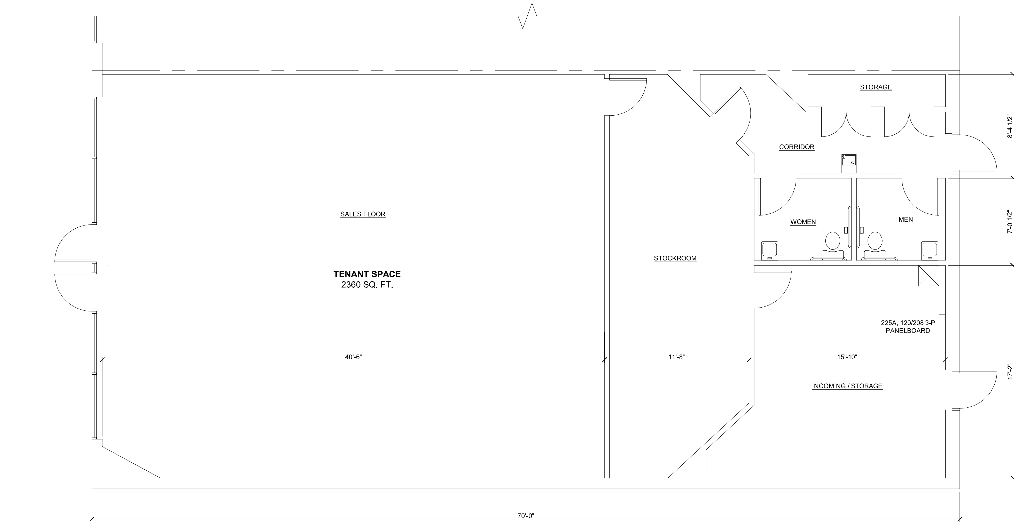
TENANT FLOOR PLAN SCALE: 1/4" = 1'-0"
