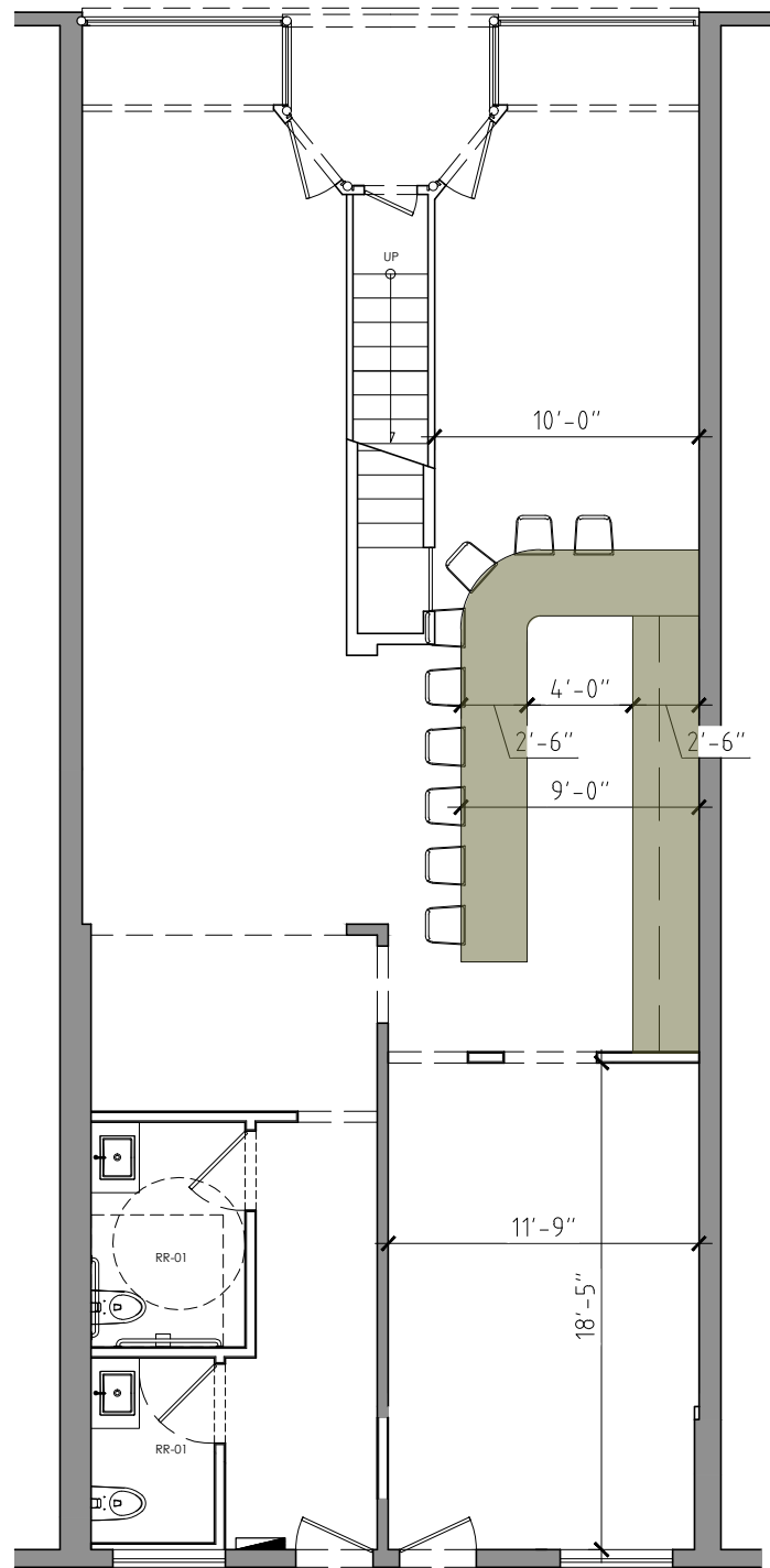
02 main floor plan 1/8" = 1'-0"
