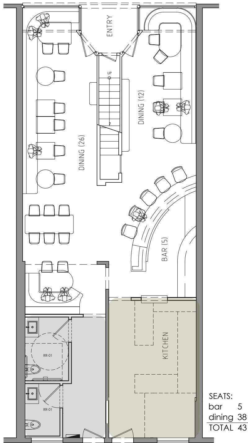
05 main floor plan 1/8" = 1'-0"
