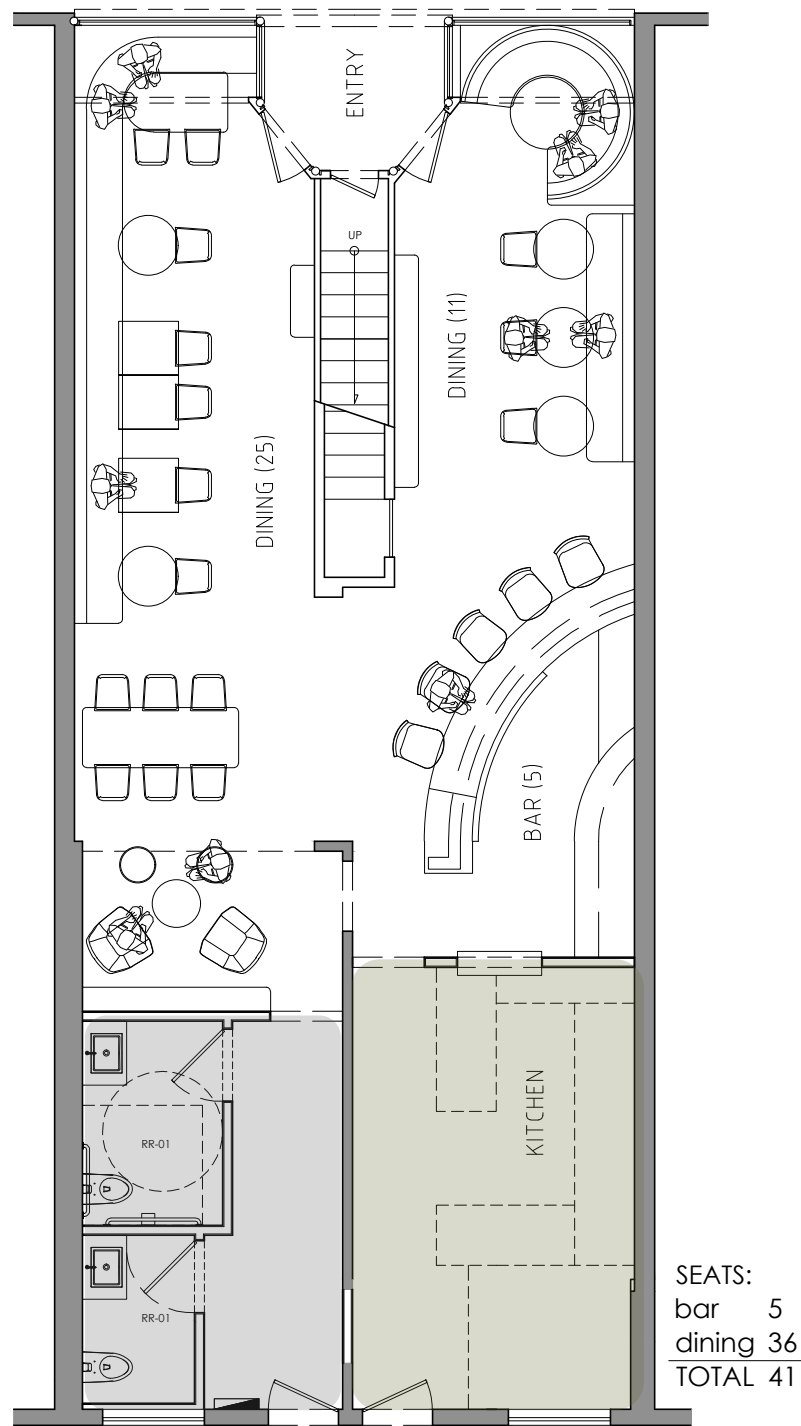
04 main floor plan 1/8" = 1'-0"
