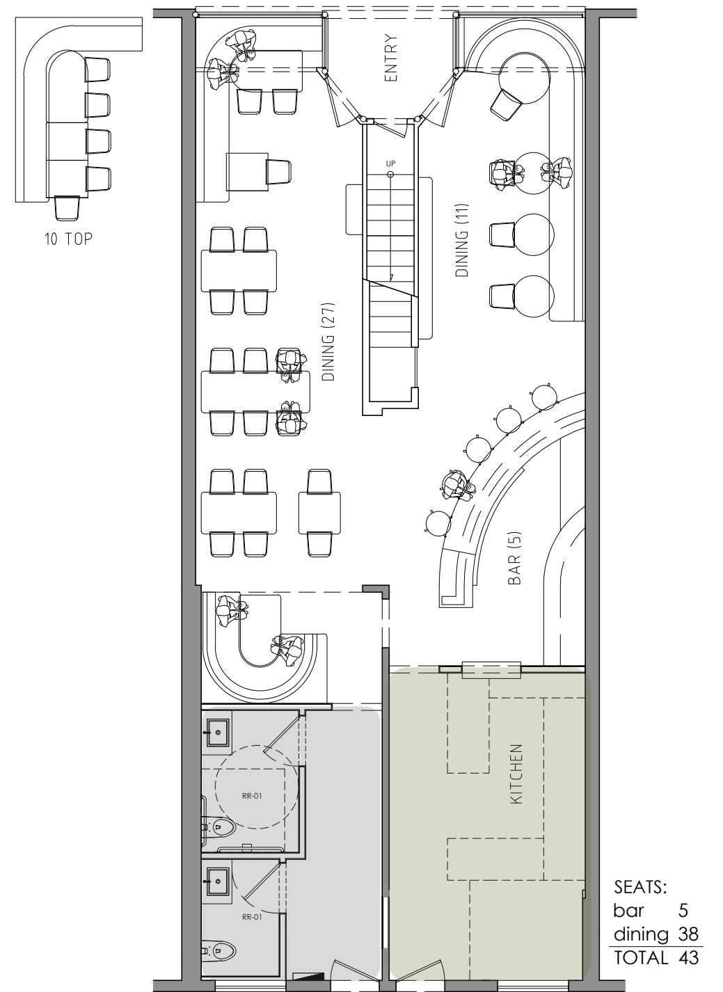
03 main floor plan 1/8" = 1'-0"
