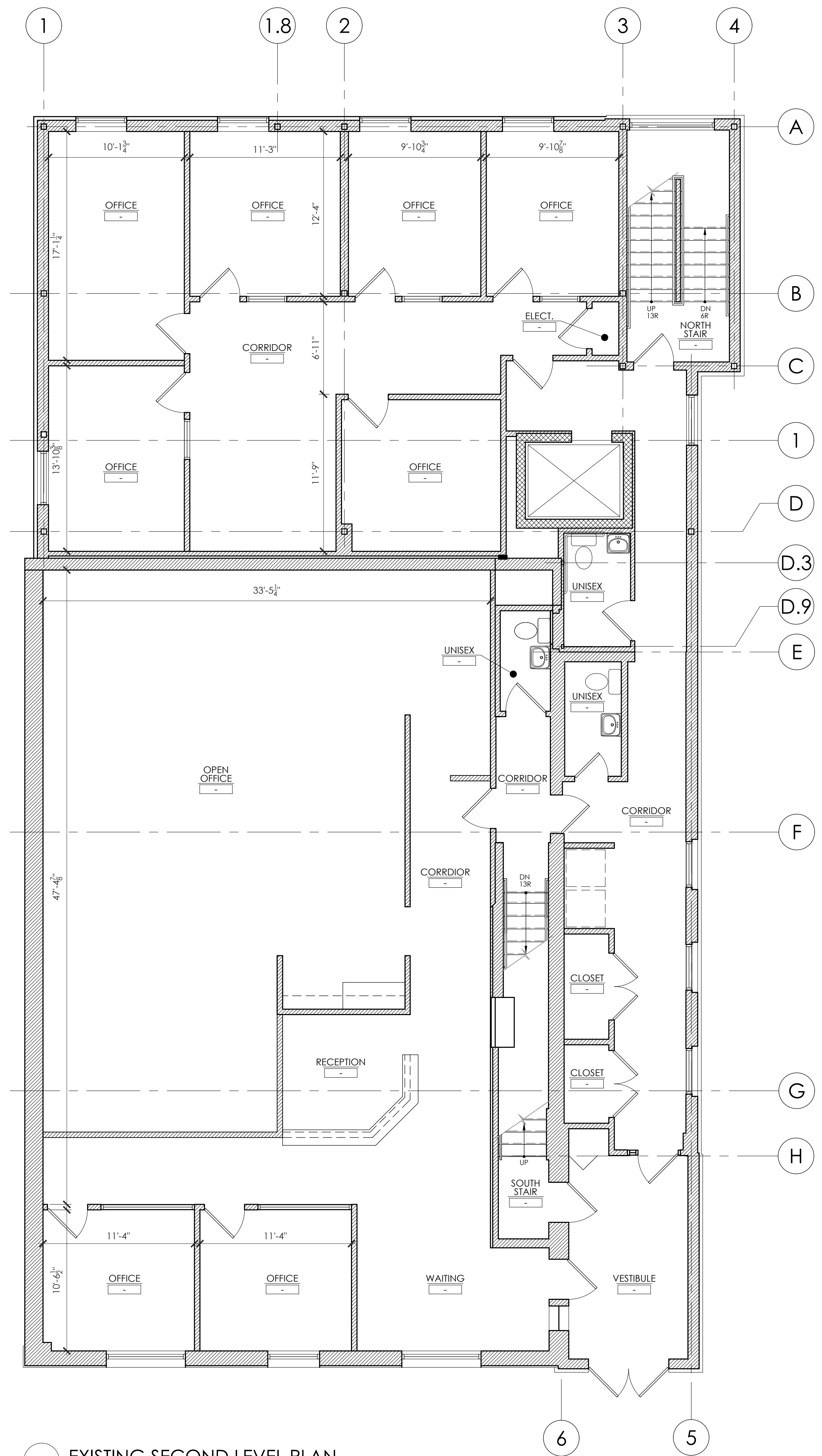
EXISTING SECOND LEVEL PLAN SCALE: 1'-0" = 3/16"
