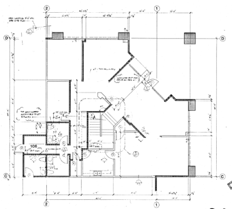
FIRST FLOOR OFFICE PLAN
