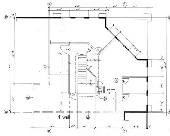
SECOND FLOOR OFFICE PLAN
