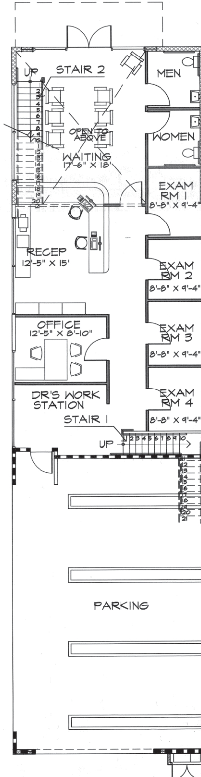
FIRST FLOOR
