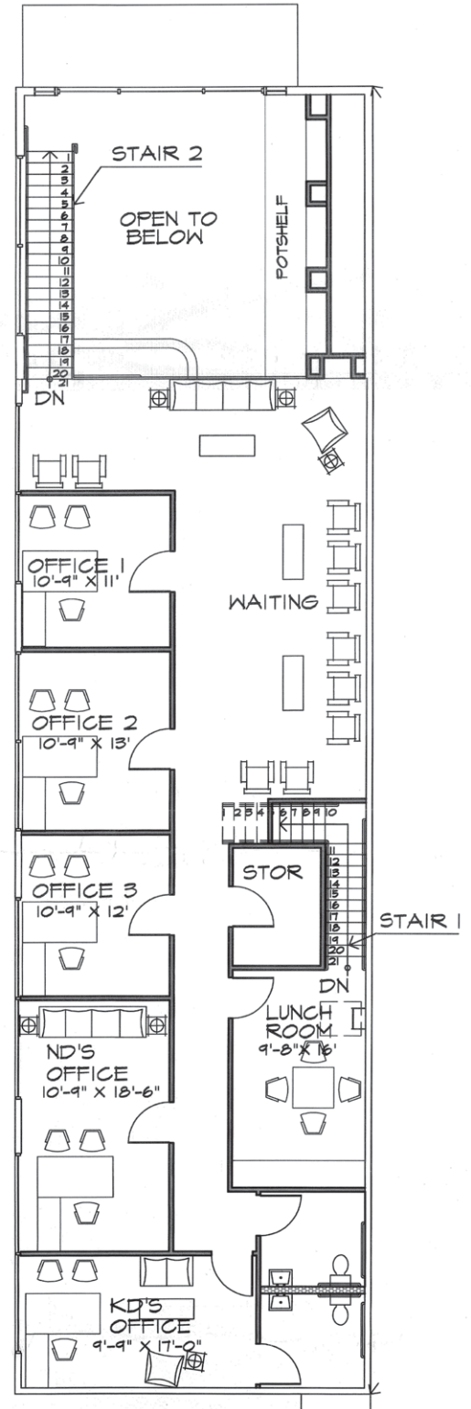
SECOND FLOOR
