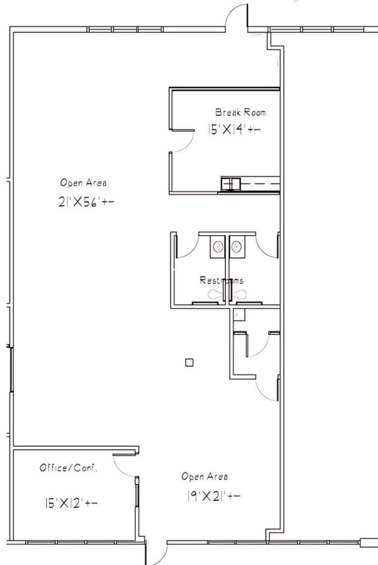
FLOOR PLAN
