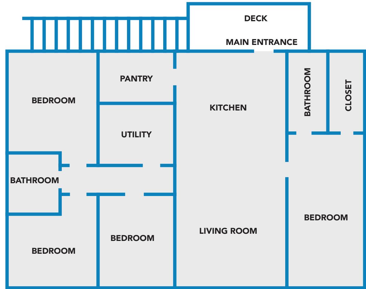
UPPER LEVEL
