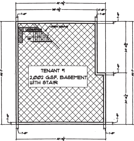
LOWER LEVEL
